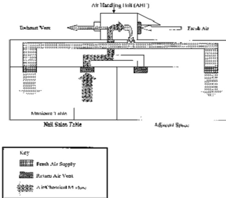
Figure 1 Transport of Odors from Nail Salon to Adjacent Space by Ventilation System
